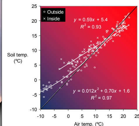
Fig. 3. Relationships between mean daily soil and air temperatures inside (upper equation) and outside a Kentucky high tunnel.
