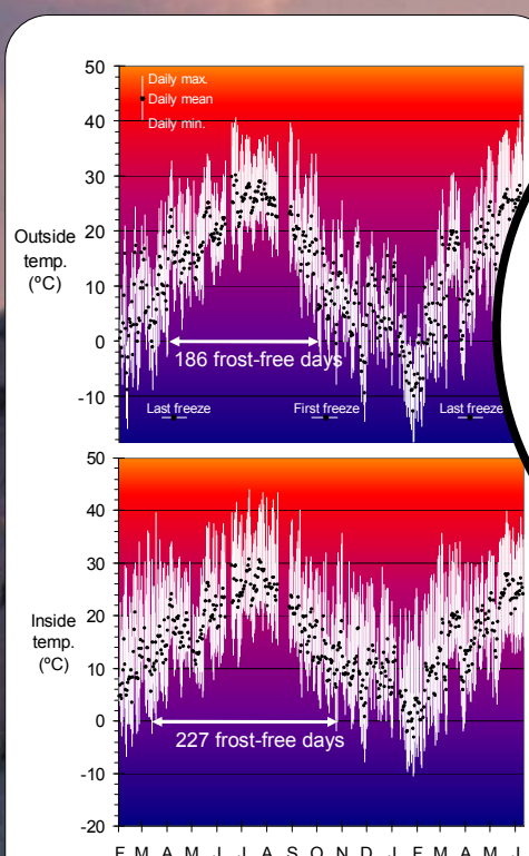
Fig. 1. Daily air temperature readings outside (top) and inside a Kentucky high tunnel from Feb. 2006 to Jun. 2007. Dots show daily mean; vertical lines show range. Average first and last freeze dates (1971-2000) are near the bottom of the upper chart, with horizontal lines depicting 90% confidence intervals. The 'close-up' magnifying glass shows air and soil temperature fluctuations over five days in April 2007 when consecutive nightly frosts following unseasonably warm weather caused severe crop damage in the region. Outdoor temperatures (blue) are compared with temperatures inside the high tunnel (green) and temperatures beneath Reemay row covers inside the tunnel (orange).
