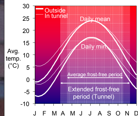
Fig. 4. Predicted mean and minimum daily temperatures inside a Kentucky high tunnel (thin line), based on observed mean and minimum daily temperatures outdoors (1970-2000; thick line) and the relationships presented in Fig. 2. Heavy and light shading shows expected frost-free periods outdoors and in the high tunnel, respectively.
