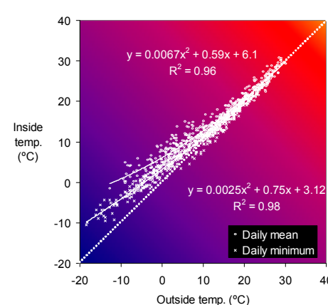
Fig. 2. Relationships between temperature outside and inside a Kentucky high tunnel. Upper and lower equations describe relationship for daily means and minima, respectively.
